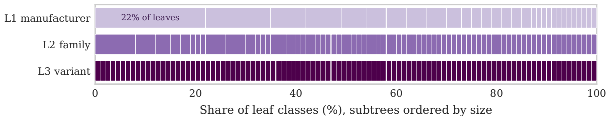
Aircraft (30→70→100)
