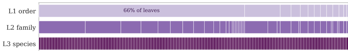
Aircraft (30→70→100)
