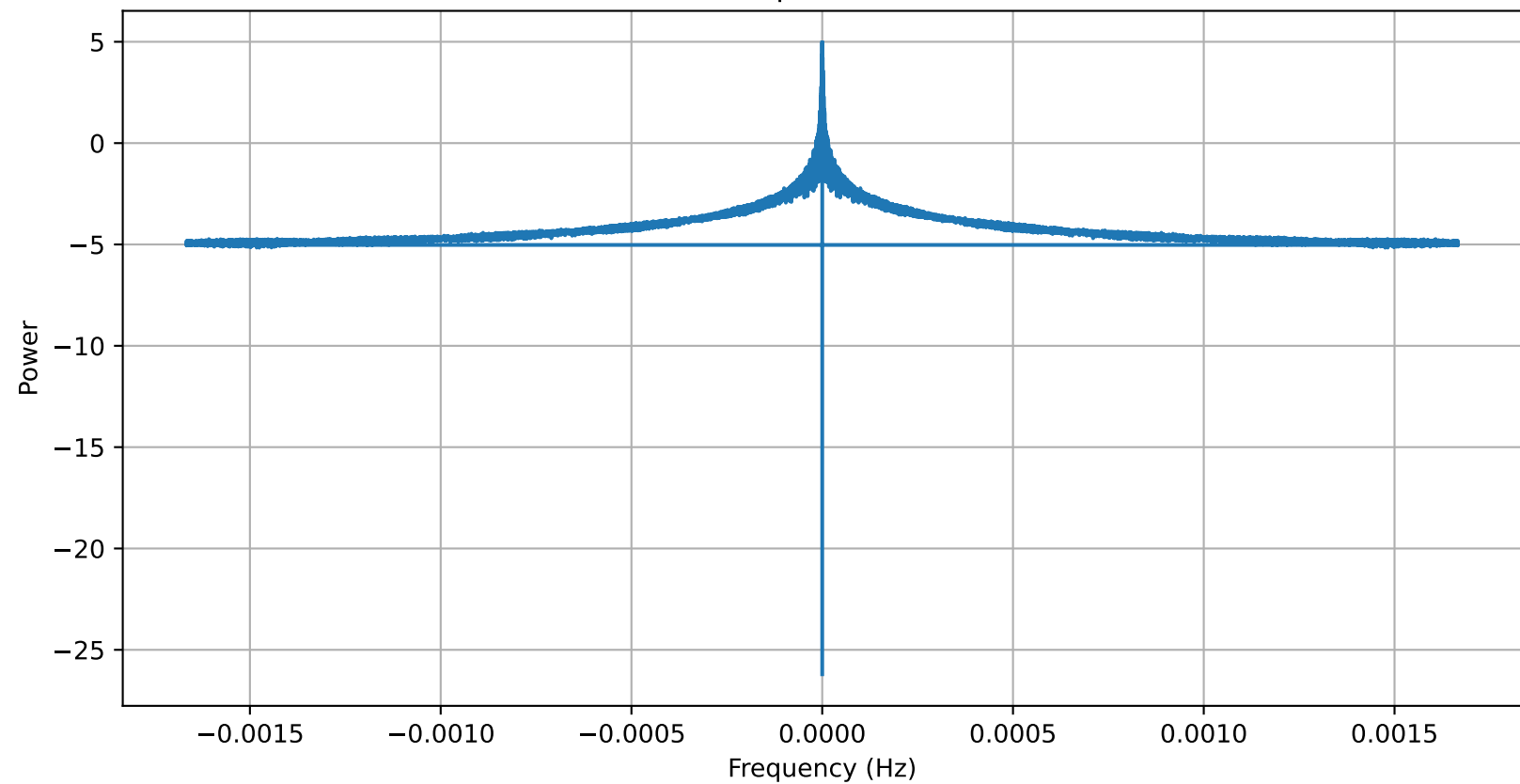
RAW ZTD Power Spectrum for 21-12-2025
