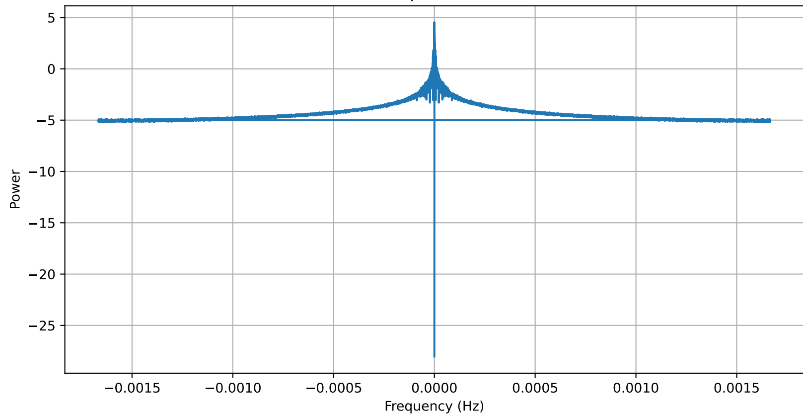
RAW ZTD Power Spectrum for 22-12-2025
