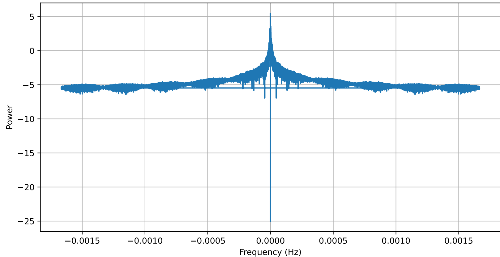
RAW ZTD Power Spectrum for 24-12-2025
