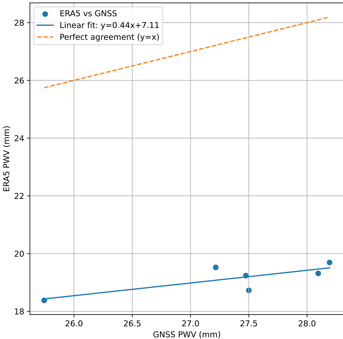
GNSS PWV vs ERA5 PWV - 23122025
