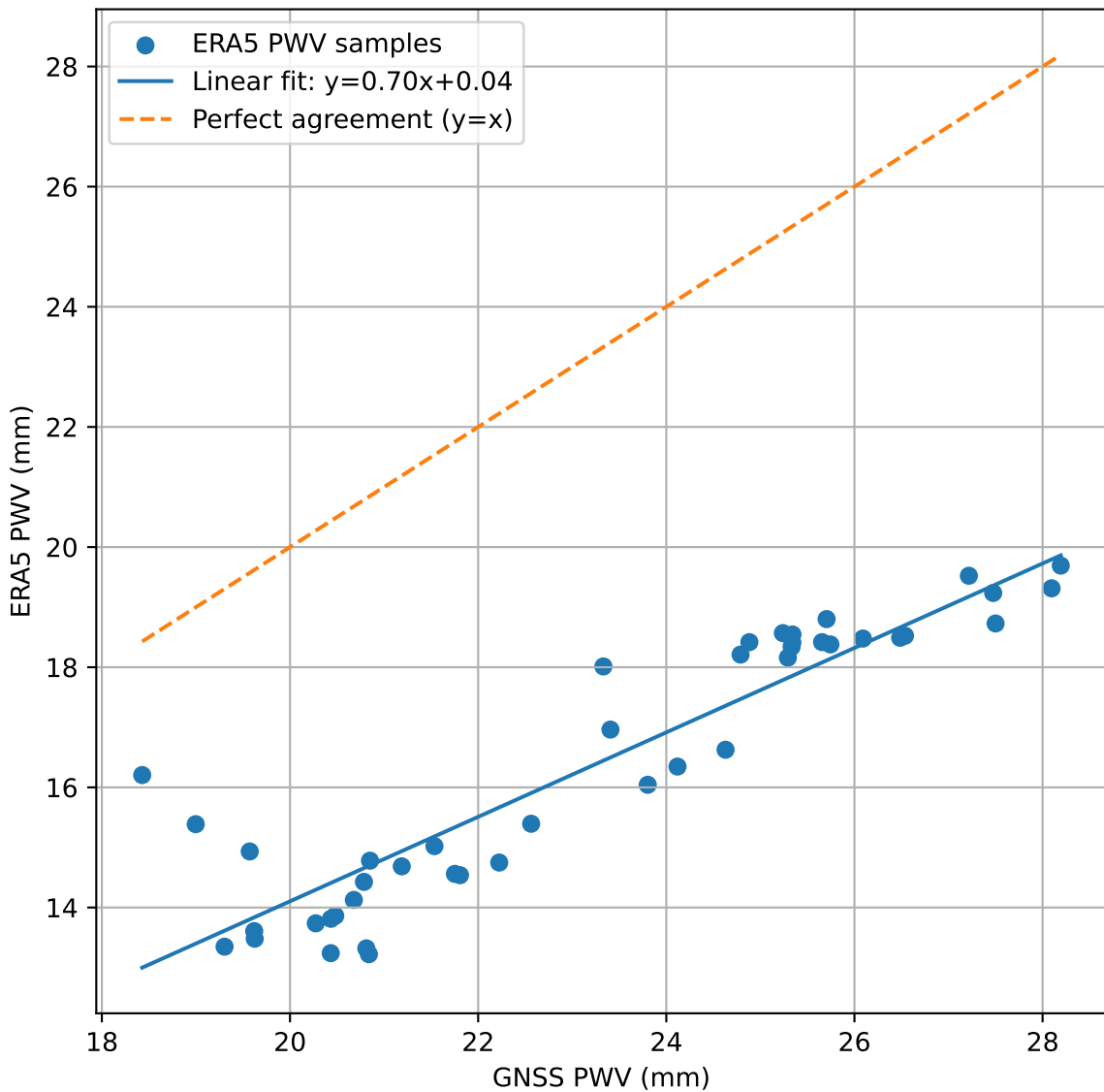
GNSS PWV vs ERA5 PWV - All Data
