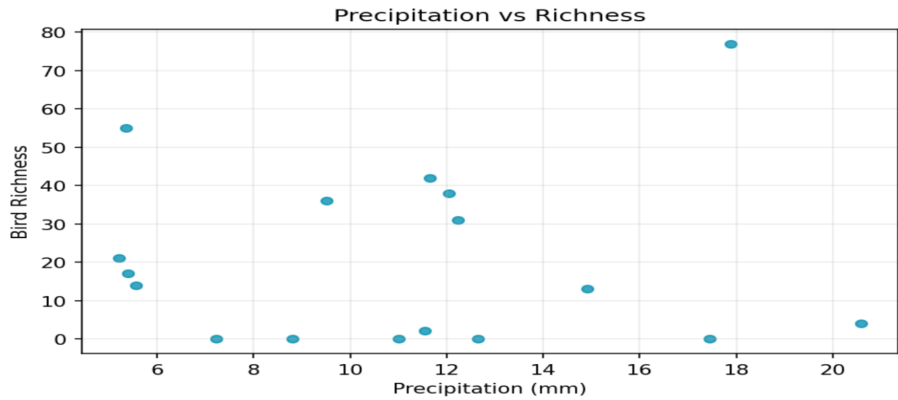
Chart: Precipitation vs Richness
