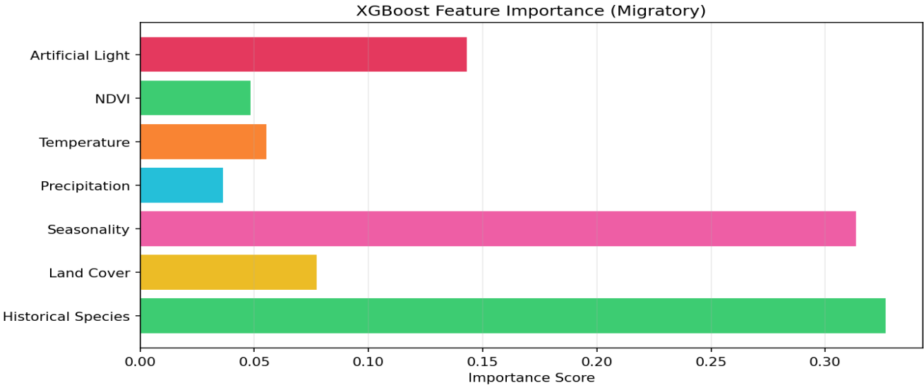
Chart: XGBoost Feature Importance (Migratory)
