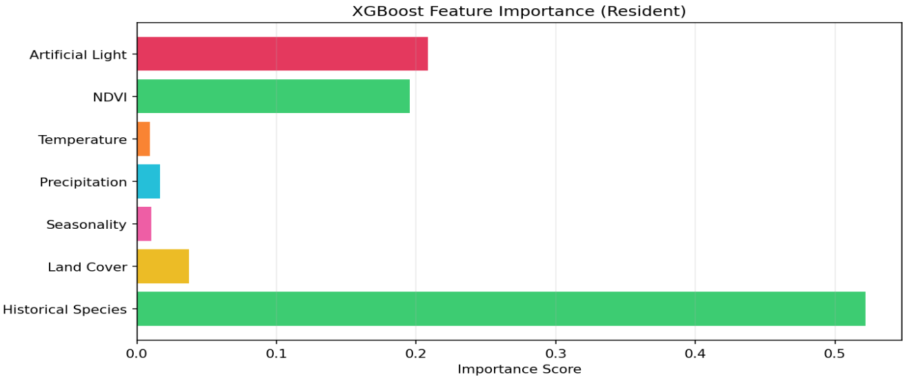
Chart: XGBoost Feature Importance (Resident)
