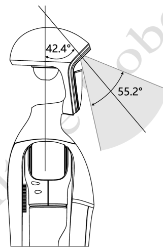
D435i Depth Camera FOV
