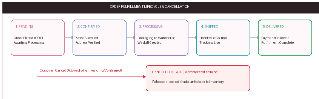
Figure 4.2: Order Fulfillment Lifecycle &amp; Customer Cancellation State Machine
