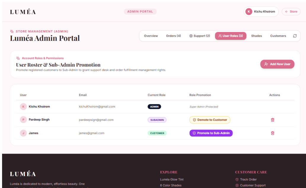
Figure 7.9: Admin Role-Based Access Control — Promoting Users to Sub-Admin
