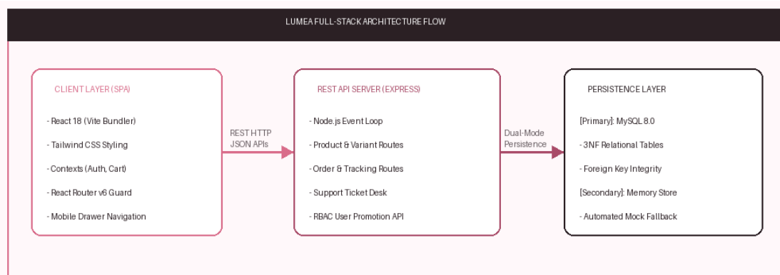
Figure 4.1: Luméa Decoupled Client-Server Architecture & Request Flow
