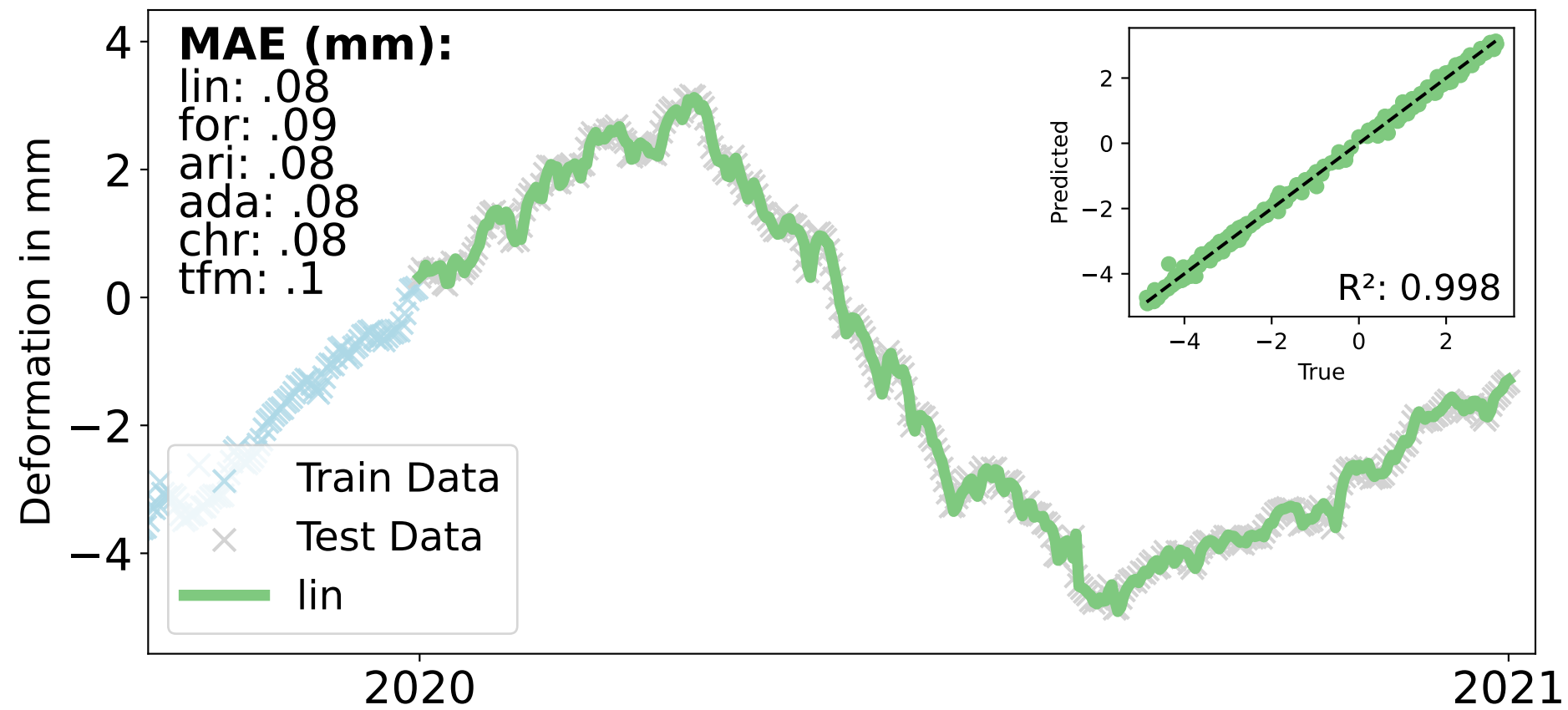
Univariate
