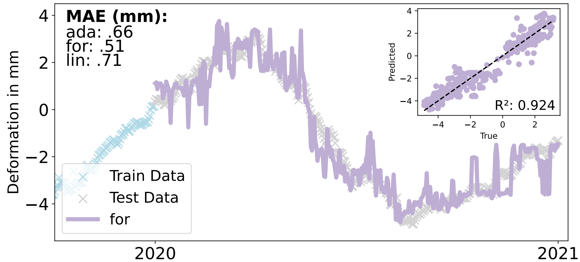
Univariate
