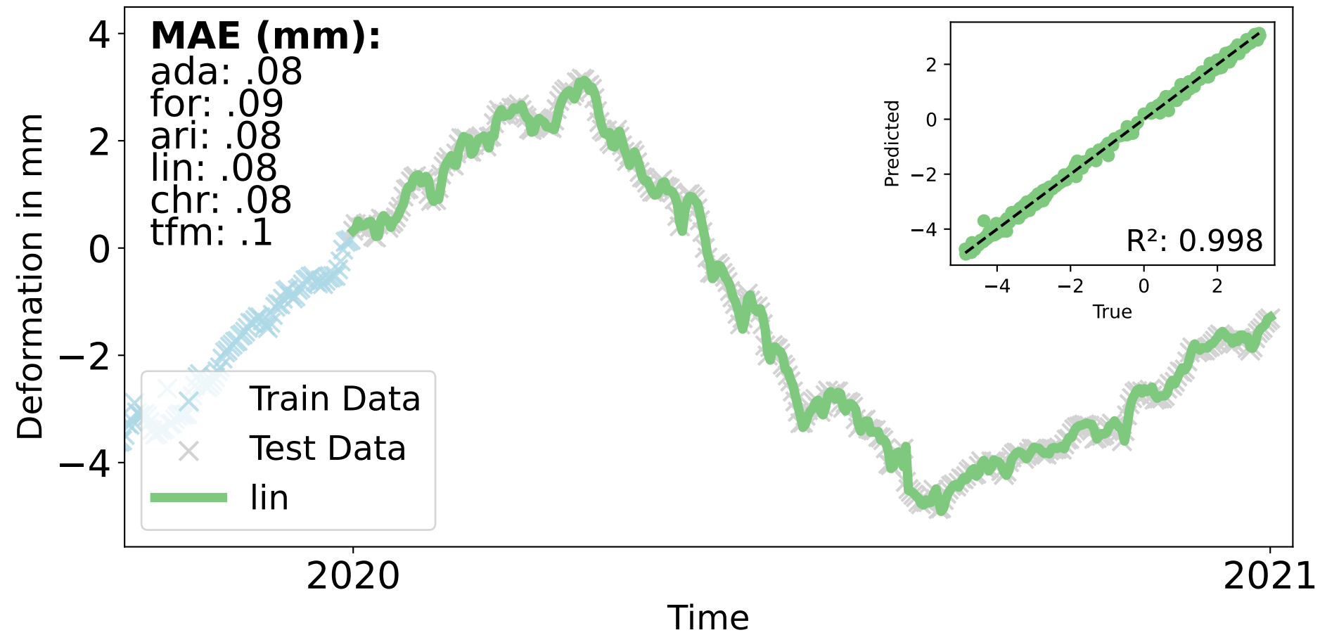
Univariate
