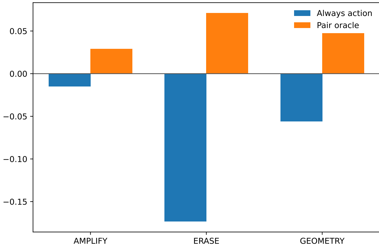
Subject-balanced \Delta BA
