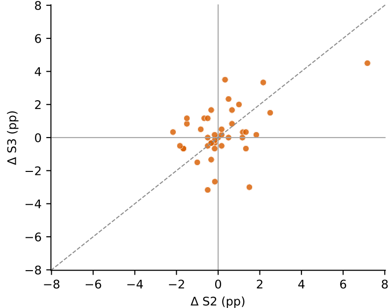
EEGConformer (Spearman 0.31)
