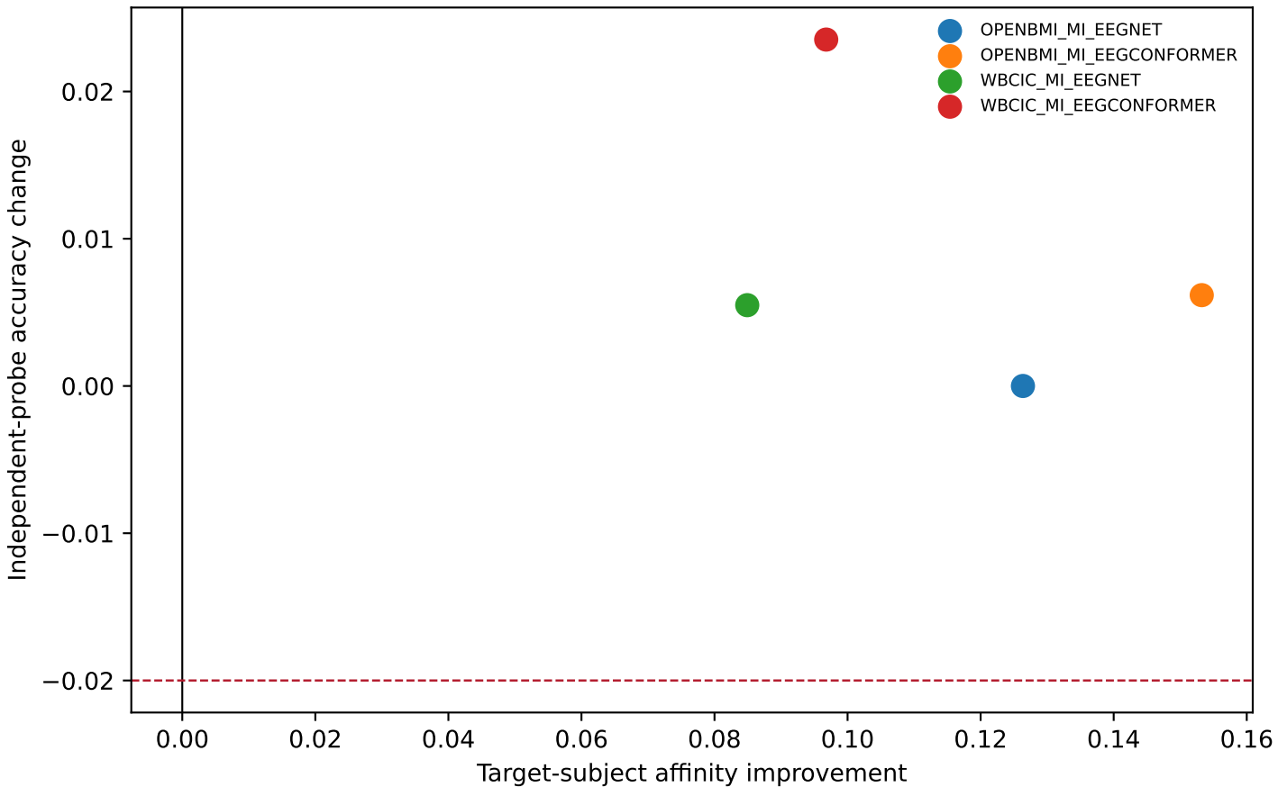
Repair-2 subject fidelity versus class fidelity
