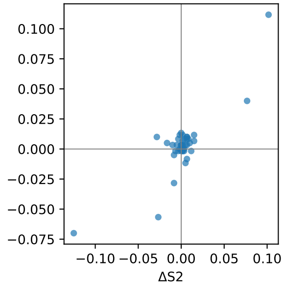
LaBraM
