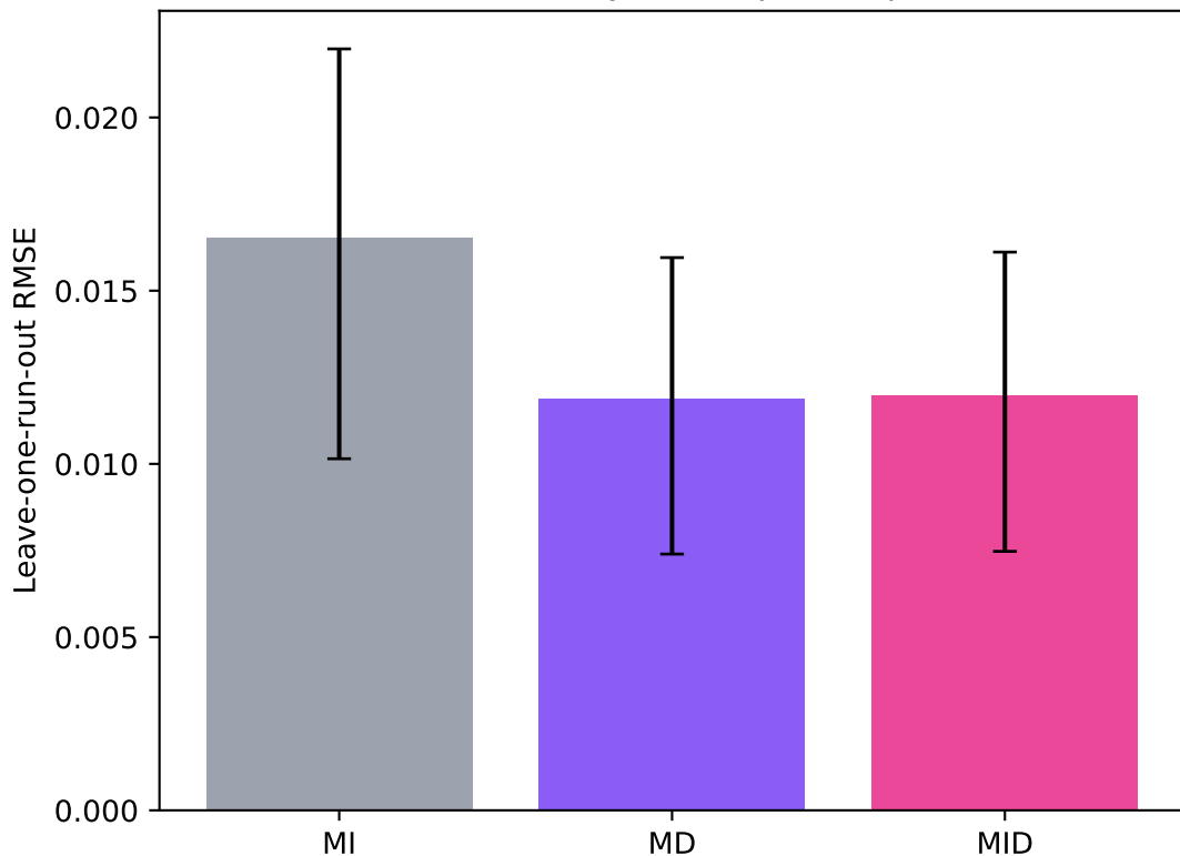
Decision vs identity consequence prediction
