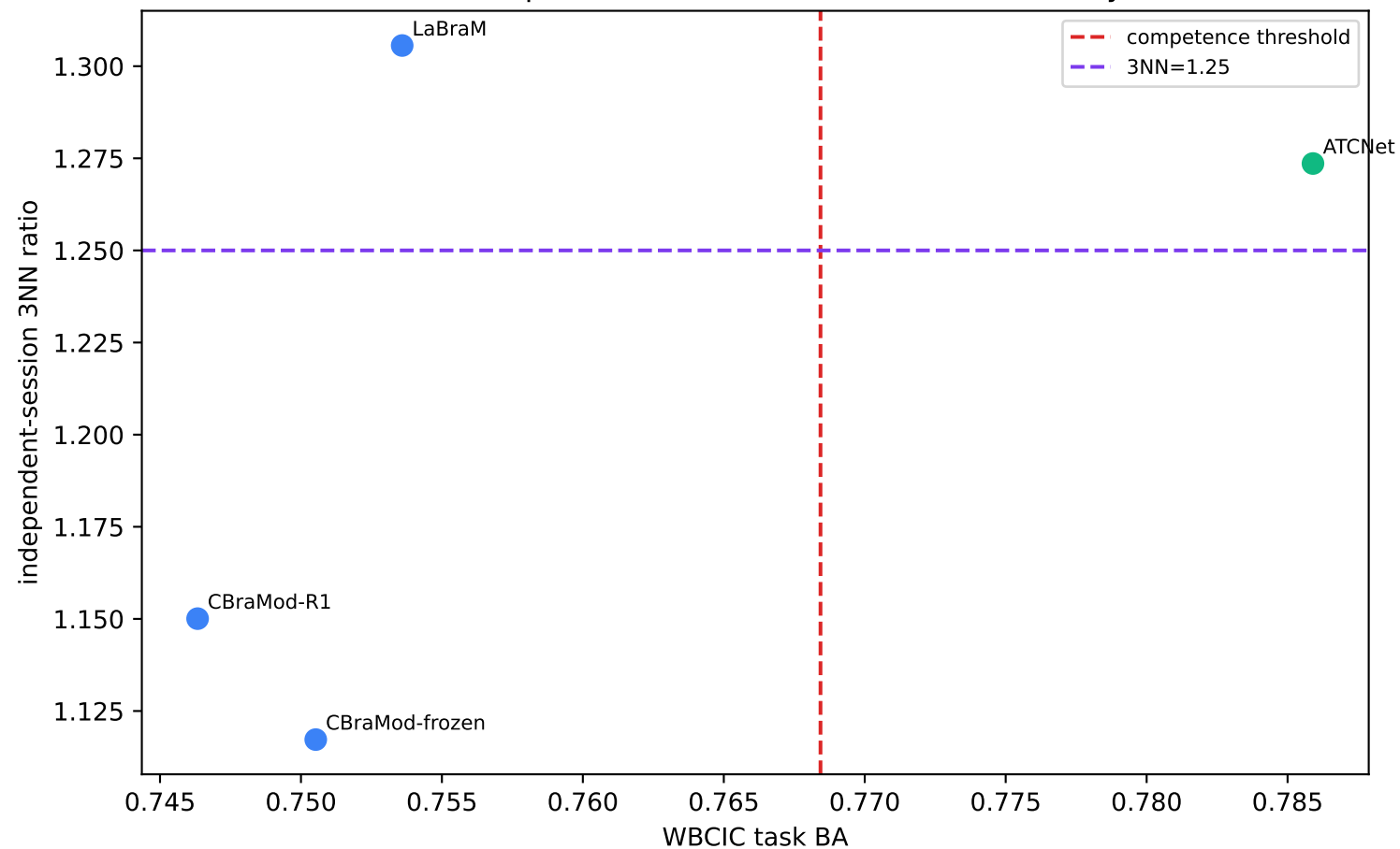
Task competence versus WBCIC manifold validity
