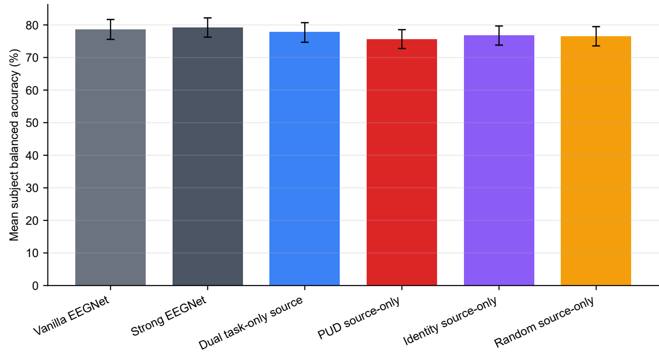
Frozen source-only Session-2 evaluation (40 subjects; 3 seeds)
