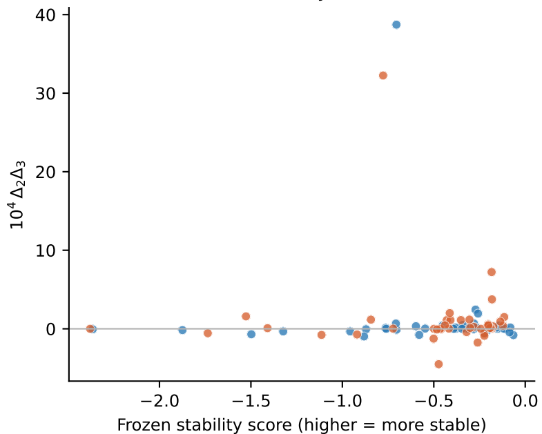
EEGConformer Decision stability ( \rho=0.22 )
