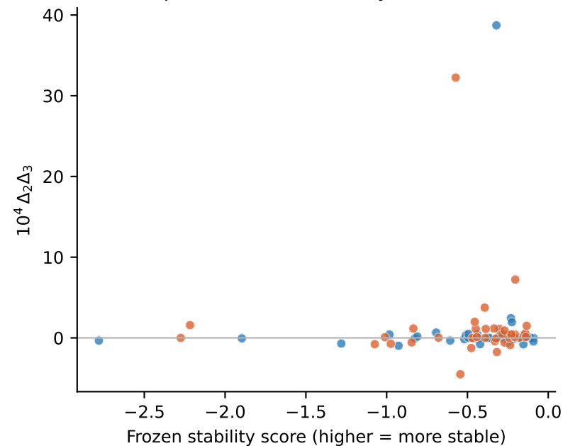
Adaptation-effect stability ( \rho=0.15 )
