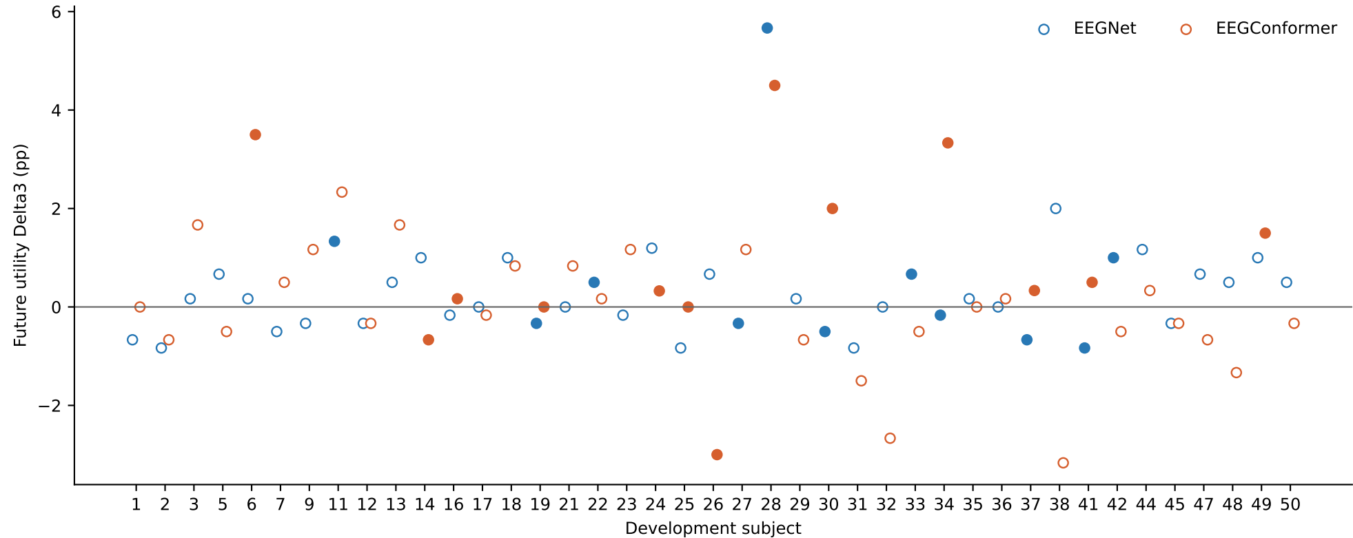
Reliability-gated decisions (filled = adapted)
