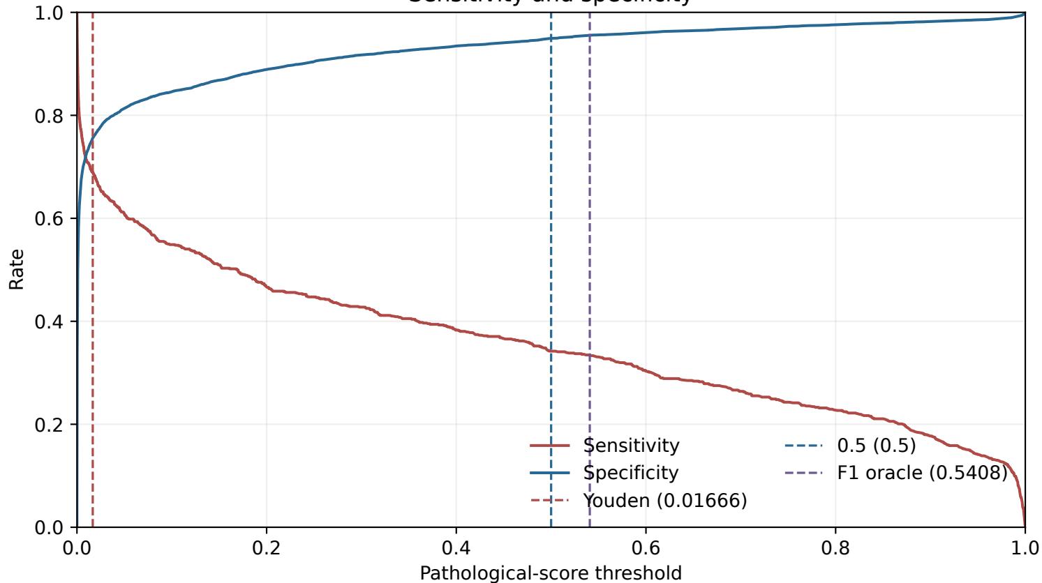
Sensitivity and specificity
