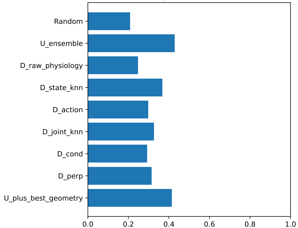
High-error AUPRC
