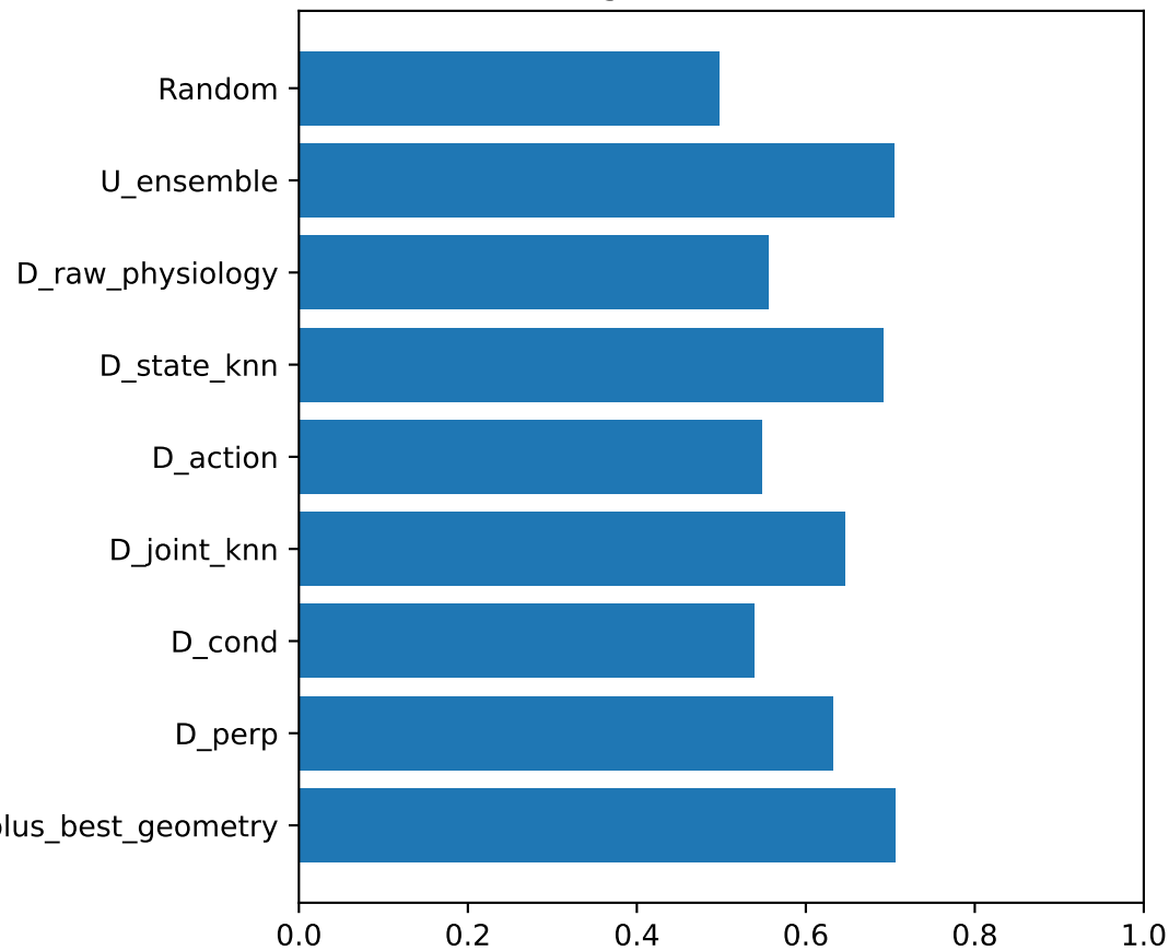
High-error AUROC
