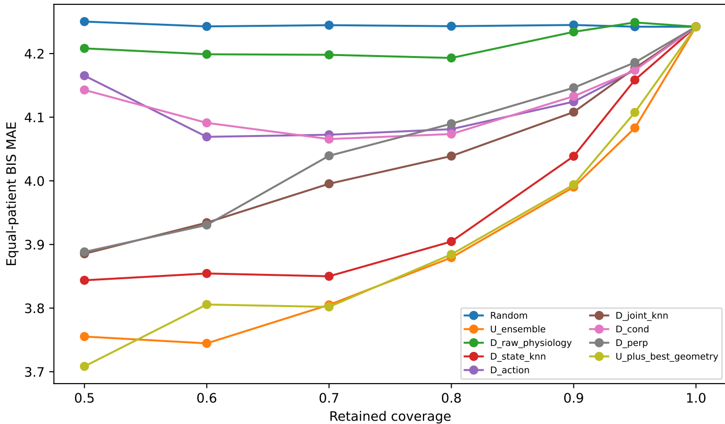
Risk-coverage
