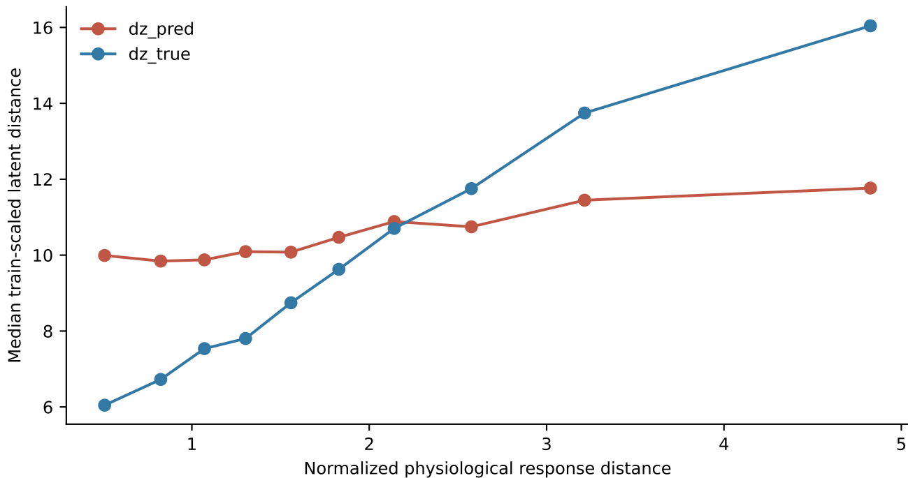
Patient-balanced sampled pairs, 300 s
