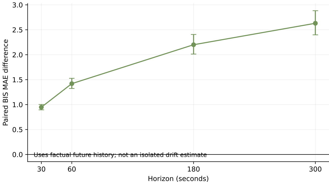
Factual-anchor Oracle-State difference
