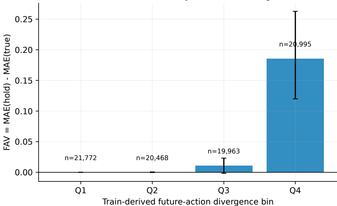
Future-action value by schedule divergence
