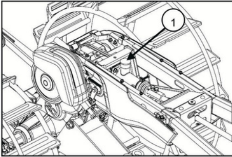
(1) Kichujio cha mafuta ya upitishaji
