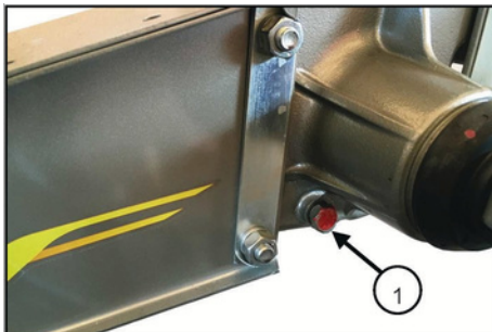
(1) Kizibo cha kukagua kiwango cha mafuta
