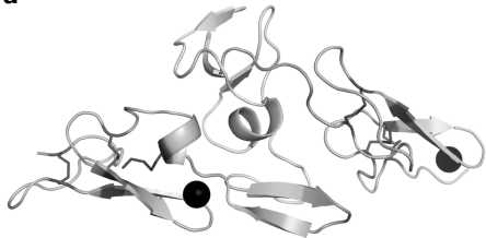
cbEGF9-hybrid 2-cbEGF10, PDB 2W86
