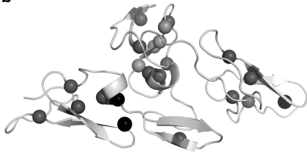
30 pathogenic variants, 20 positions
