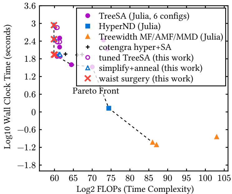
Sycamore 53q, m=20 (3369 tensors)
