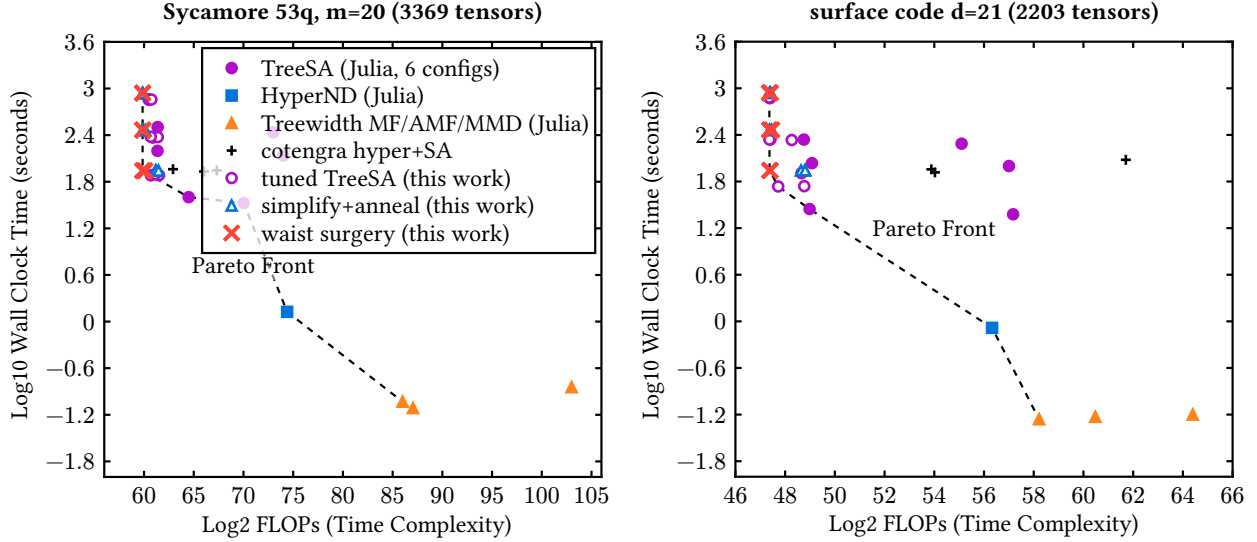
Figure 9: Time-versus-quality Pareto view of the same-machine campaign (dedicated 2-core server, all runs single-threaded), in the presentation style of the OMEinsumContractionOrders benchmark study [6]. Each point is one optimizer configuration or repetition: filled markers are external baselines (Julia TreeSA ladder, HyperND, treewidth back-ends, cotengra hyper-optimizer with SA refinement); open markers are this work at 90/300/900s budgets. The dashed line is the non-dominated front. Waist surgery (stars) holds the entire high-quality wall of the front on both instances.
