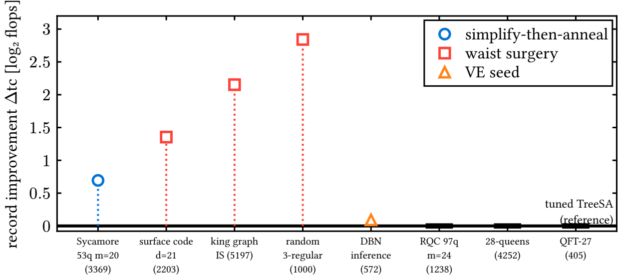
Figure 8: The record board: confirmed improvement over the tuned TreeSA reference on each instance (validator protocol: confirm-twice, worse-of-two, per-run relabeling). Marker shape and color encode the winning mechanism; horizontal dashes mark instances where the tuned reference is the record holder.
