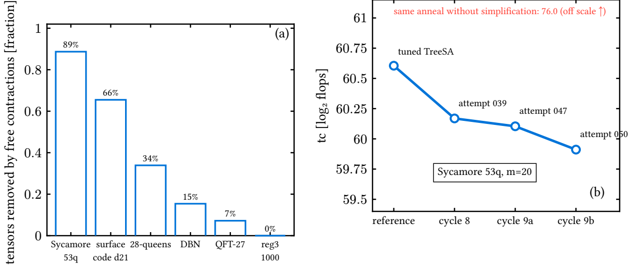
Figure 6: Structural simplification. (a) Fraction of tensors removed by the exact rank-non-increasing pass; the random-regular control is untouched at 0%. (b) The Sycamore 53q record march: the tuned reference (leftmost) and three successive simplify-then-anneal attempts. The same anneal without simplification reaches 76.0 (off scale): preprocessing, not search, carries the improvement.
