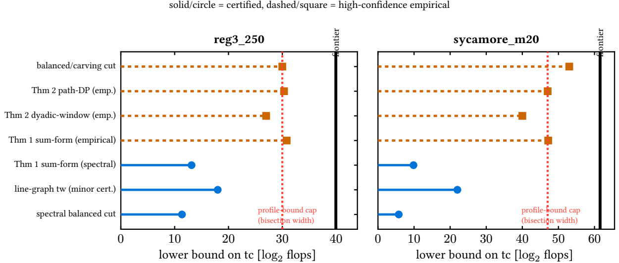
Figure 3: Lower-bound ladder for both closed instances. Solid stems with circles are certified (machine-checkable certificates); dashed stems with squares are high-confidence empirical values. Every profile-based bound (Theorems 1 and 2) is capped at the bisection width (dotted line, Observation 1); only the balanced/carving cut exceeds it. The solid vertical line is the optimizer frontier.
