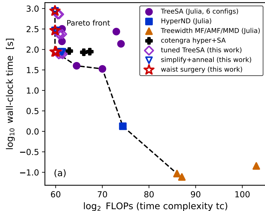
Sycamore 53q, m=20 (3369 tensors)
