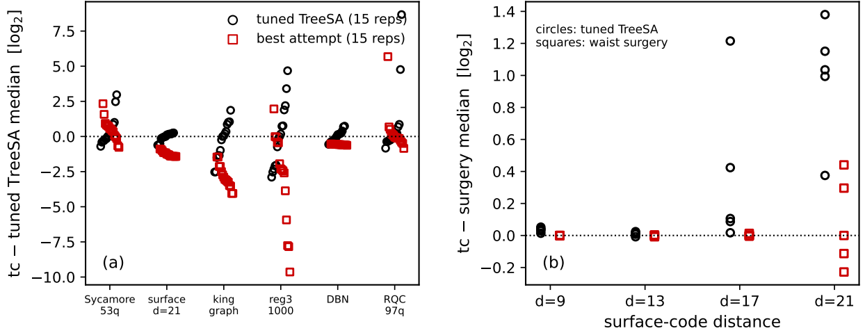
Figure 10: Statistical view of the same-machine campaign. (a) All 15 repetitions per instance at 90 s, centered on the tuned reference’s median: circles are the tuned reference, squares the best attempt per instance. (b) Surface-code family: repetitions at 90 s versus code distance, anchored at the surgery median per distance; the advantage grows with d while the surgery spread stays collapsed.
