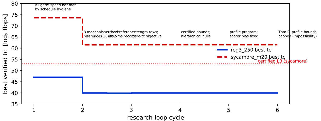
Figure 12: Best verified tc over the research-loop cycles. Apparent progress in cycle 2 is reclaimed by the strengthened reference (cycle 2.5); thereafter the closed-instance frontier is flat while the certified picture grows, and cycles 7–10 move the record board on the large structured instances instead. Annotations mark the three instrument-caught failure modes.
