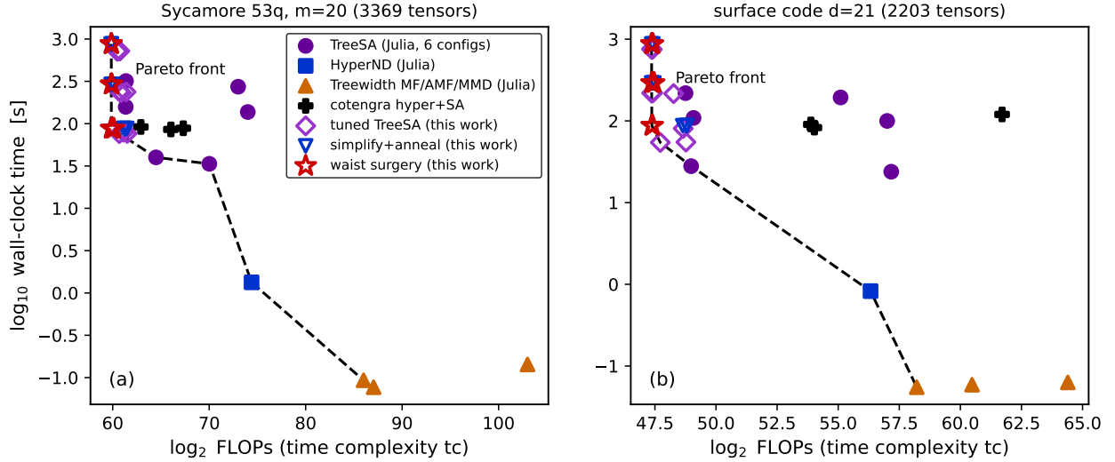
Figure 9: Time-versus-quality Pareto view of the same-machine campaign (dedicated 2-core server, all runs single-threaded), in the presentation style of the OMEinsumContractionOrders benchmark study [6]. Each point is one optimizer configuration or repetition: filled markers are external baselines (Julia TreeSA ladder, HyperND, treewidth back-ends, cotengra hyper-optimizer with SA refinement); open markers are this work at 90/300/900s budgets. The dashed line is the non-dominated front. Waist surgery (stars) holds the entire high-quality wall of the front on both instances.
