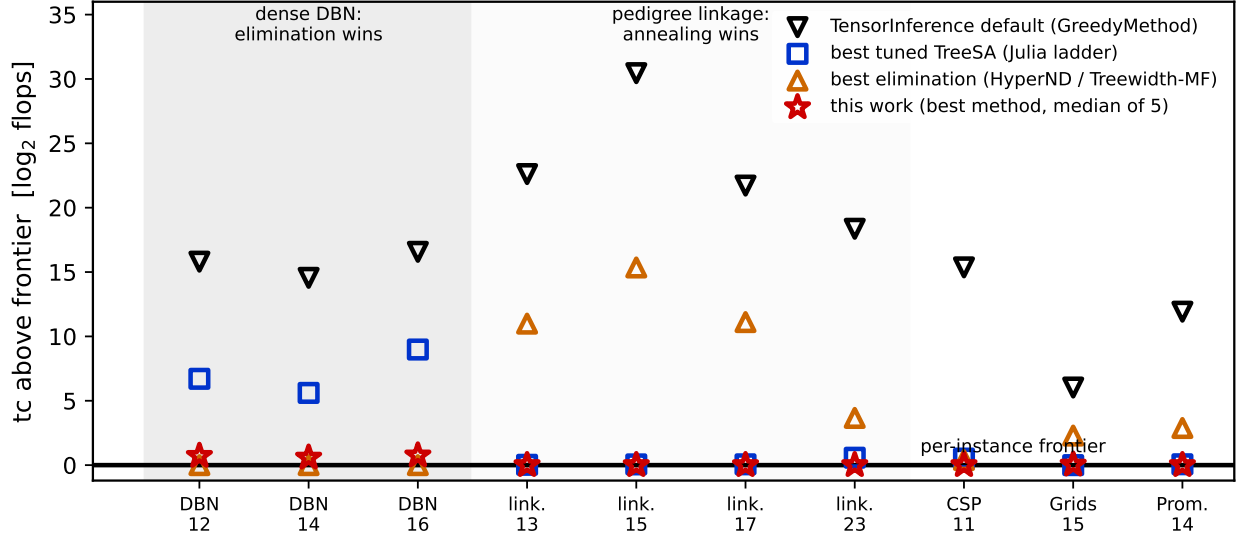
Figure 11: The ten hardest UAI-2014 MAR instances (from a 65-instance scan): each method’s tc above the per-instance frontier, same machine, 90 s budgets for search methods. Down-triangles: TensorInference.jl’s signature default. Squares: best tuned TreeSA from the Julia ladder. Up-triangles: best elimination method (min-fill treewidth / HyperND; KaHyPar segfaults on all four linkage instances, so its rows there are min-fill only). Stars: this work (best method, median of five). Shaded bands mark the two regimes.
