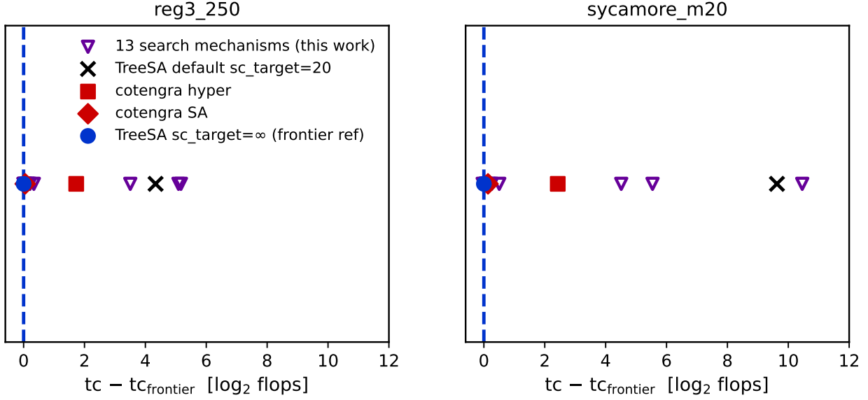
Figure 2: Distance of every scored optimizer from the frontier value (dashed line at zero). Open triangles: the thirteen search mechanisms of this work. Filled symbols: the tuned TreeSA reference ( sc_{\text{target}} = \infty , circle), cotengra’s SA refiner (diamond), cotengra’s hyper-optimizer (square), and the shipped-default TreeSA (cross).
