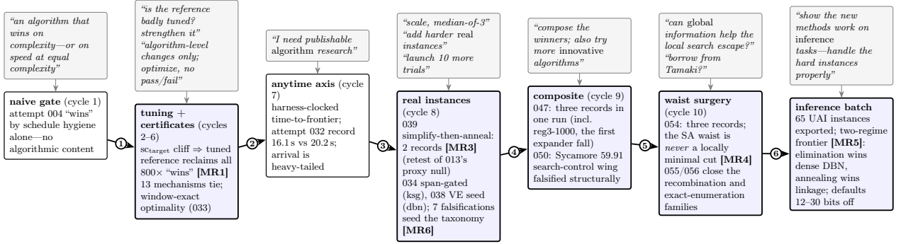
Figure 13: The research roadmap, left to right. Top row (grey): the human steering prompts, essentially verbatim. Bottom row: the result-carrying attempts only (shaded boxes contain main results); most of the 56 attempts are controls and falsifications that feed Table 3 and Sec. 11. Each numbered arrow is a transition forced by a measurement: (1) the gate was passed without an algorithm, so the gate was hardened and references ratcheted; (2) tc saturated and was certified locally optimal, so the objective axis changed to arrival time; (3) speed gains sat at the confirmation noise floor while scale budgets were non-converged, so the regime changed; (4) the winning mechanisms proved complementary, so they were composed while exploration continued; (5) every win injected global information as input while every search-control variant failed, so global information was aimed directly at the local search's blind spot—the dominant cut; (6) the mechanism portfolio was complete, so it was pointed at a second application domain to test transfer.
