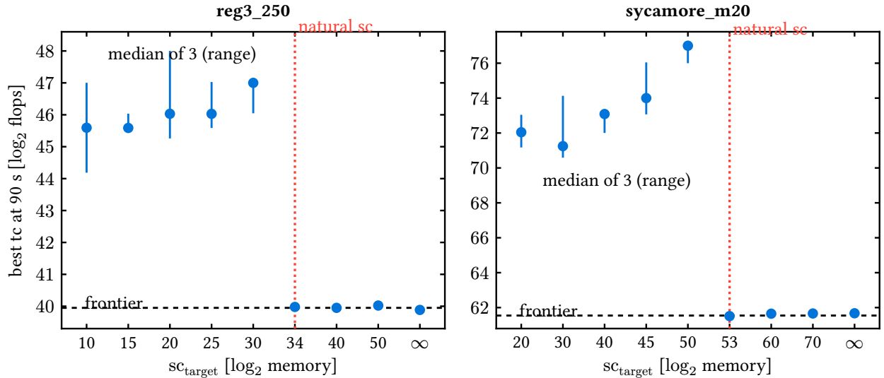
Figure 9: Best tc reached in 90s of single-threaded annealing versus the memory target sc_{\text{target}} (median of three runs; whiskers span the range). The dashed line marks the converged frontier of Appendix A; the dotted vertical line marks the natural space cost of optimum-quality trees. The transition is a cliff at the natural value: every smaller target is comparably harmful, and every target at or above it, including sc_{\text{target}} = \infty , reaches the frontier. The shipped default is sc_{\text{target}} = 20 .
