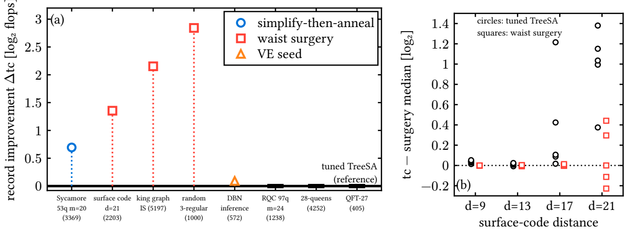
Figure 1: The advantage, summarized. (a) Record board: confirmed improvement over the tuned TreeSA reference on each instance (validator protocol: confirm-twice, worse-of-two, per-run relabeling); marker shape and color encode the mechanism, thick dashes mark instances where the tuned reference remains the record holder. (b) Surface-code family: all repetitions at 90s versus code distance, anchored at the surgery median per distance — the surgery advantage grows with d while its run-to-run spread stays collapsed.
