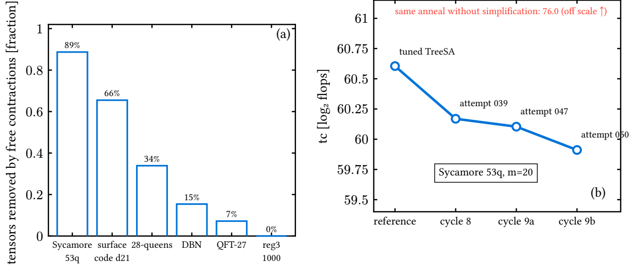
Figure 10: The preprocessing pass. (a) Fraction of tensors removed by the exact rank-non-increasing pass; the random-regular control is untouched at 0%. (b) The Sycamore 53q record march: the tuned reference (leftmost) and three successive simplify-then-anneal attempts. The same anneal without simplification reaches 76.0 (off scale): preprocessing, not search, carries this improvement.
