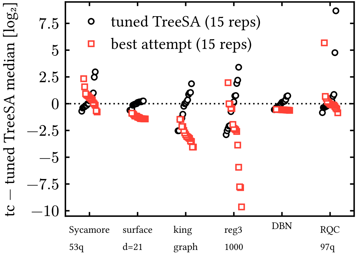
Figure 11: Run distributions of the same-machine campaign: all 15 repetitions per instance at 90 s, centered on the tuned reference's median. Circles are the tuned reference, squares the best method per instance.
