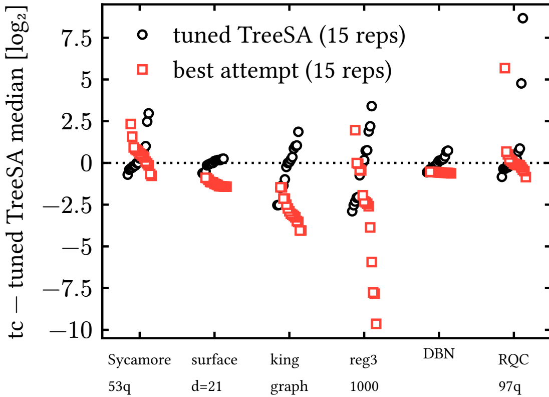
Figure 12: Run distributions of the same-machine campaign: all 15 repetitions per instance at 90 s, centered on the tuned reference's median. Circles are the tuned reference, squares the best method per instance.
