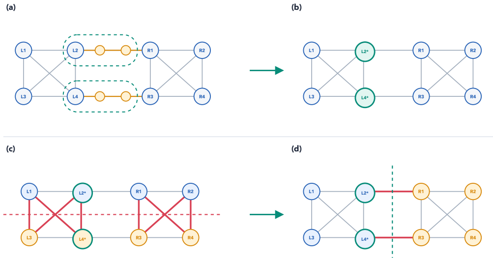
Figure 2: The two mechanisms on a toy network: two dense clusters (each a K_4 ) joined by two sparse bridges. (a,b) Preprocessing: the chain tensors on the bridges are rank-non-increasing, so the exact simplification pass absorbs them ( L_2, L_4 \rightarrow L_2^*, L_4^* ) before any search begins. (c,d) Surgery: a converged annealed tree can freeze with a poor waist—the horizontal bipartition (c), which cuts through both clusters—while the cheap comparable-balance cut through the two bridges (d) is invisible to local tree moves; bounded FM on the tensor graph finds it, and both sides are rebuilt cold and spliced.
