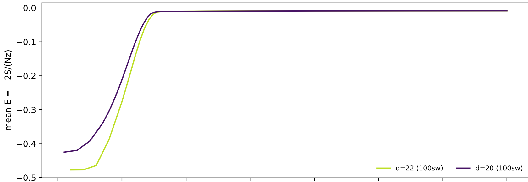
zipf_cb4 d=8..22 normalized C_S (ordered init, scaled sweeps)
