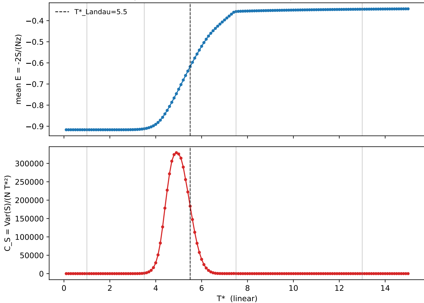
d24 geometric ordered (350+50 sweeps, ordered init)
