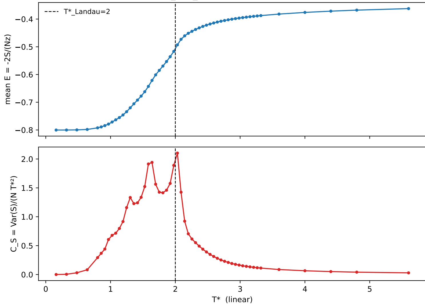
geometric_d10_ordered (300,000+50 sweeps)
