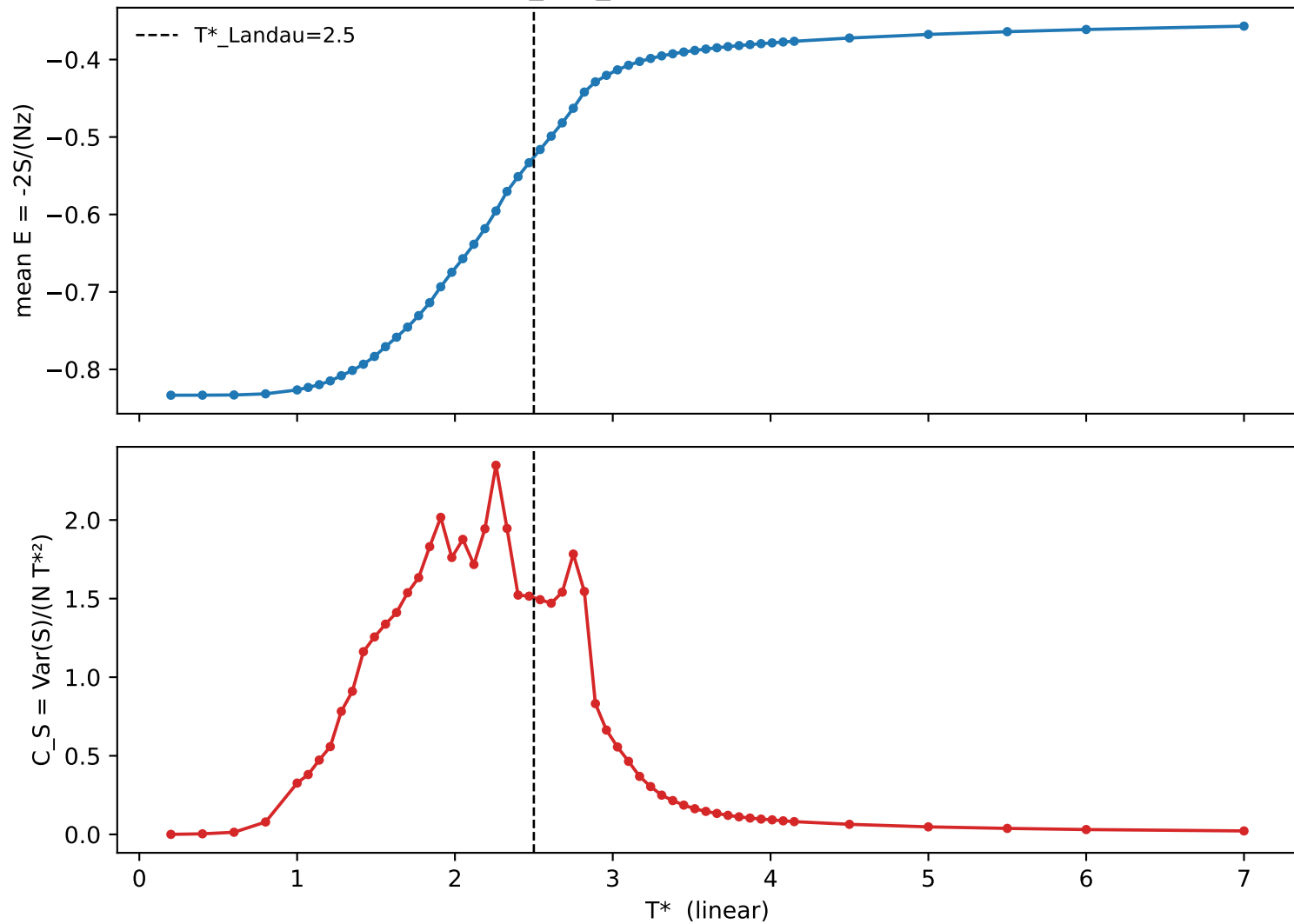
geometric_d12_ordered (80,000+50 sweeps)
