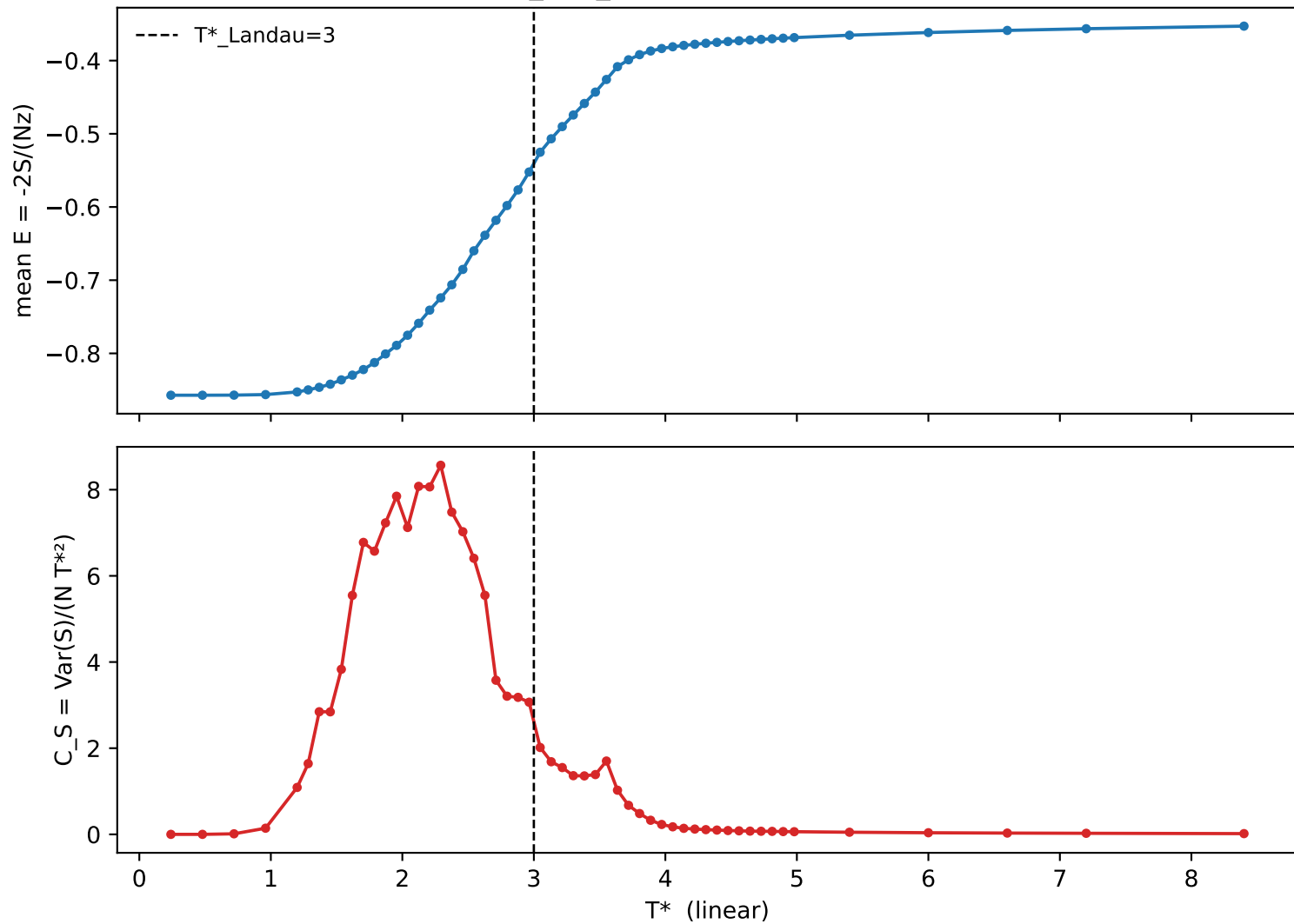
geometric_d14_ordered (20,000+50 sweeps)
