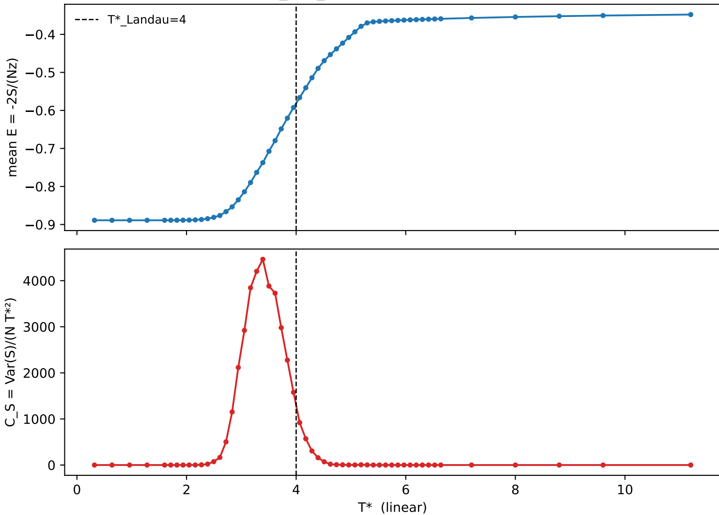
geometric_d18_ordered (d=18, 400+50 sweeps)
