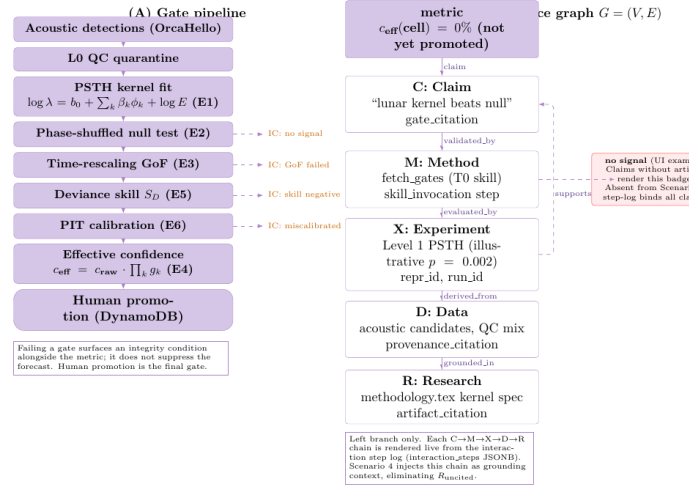
Figure 2: The mechanism that produces R_{uncited} = 0\% . (A) Gate pipeline from acoustic detections to displayed confidence. (B) Provenance graph G = (V, E) : Claim (C) → Method (M) → Experiment (X) → Data (D) → Research (R). Claims without a bound artifact render the “no signal” badge. Scenario 4 eliminates R_{uncited} because the planner step-log binds every claim to an artifact reference.
