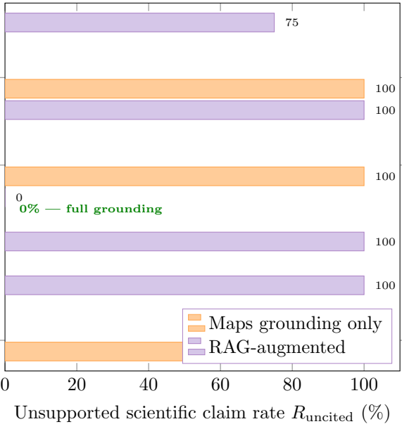
(B) R_{\text{uncited}} across 8 grounding scenarios
