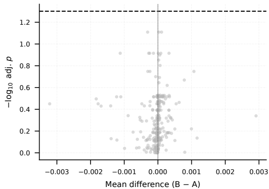
RNA
