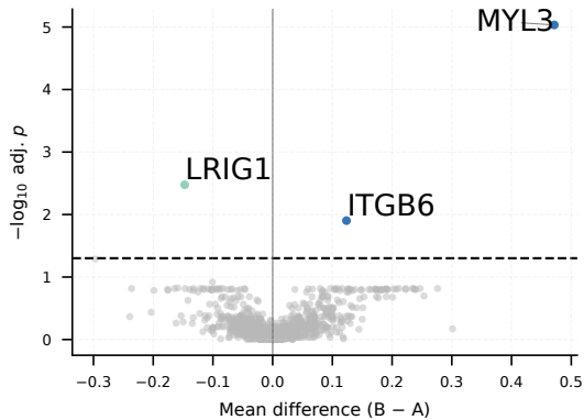
Metabolites (NMR)
