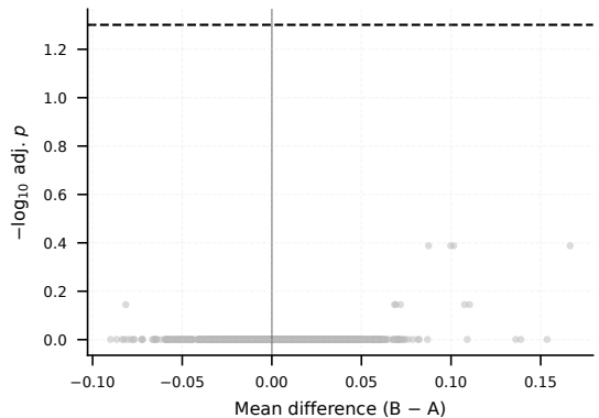
RNA
