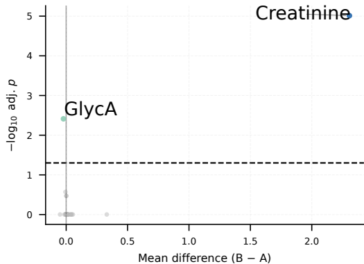
Metabolites (NMR)
