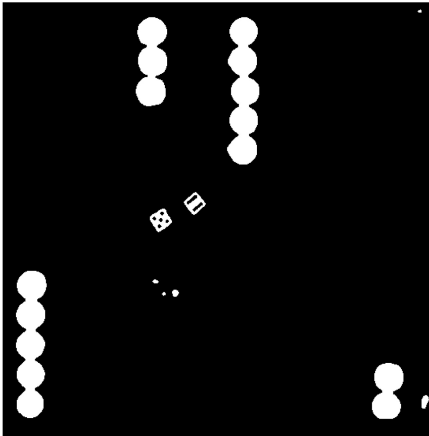
White Mask
