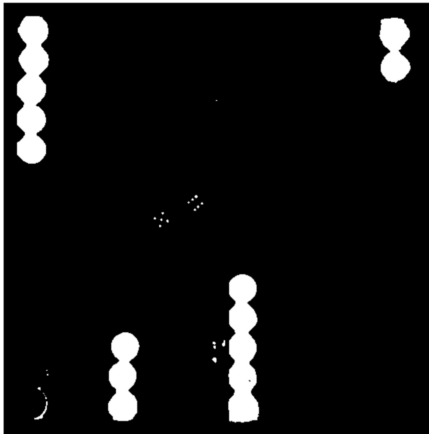
Black Mask
