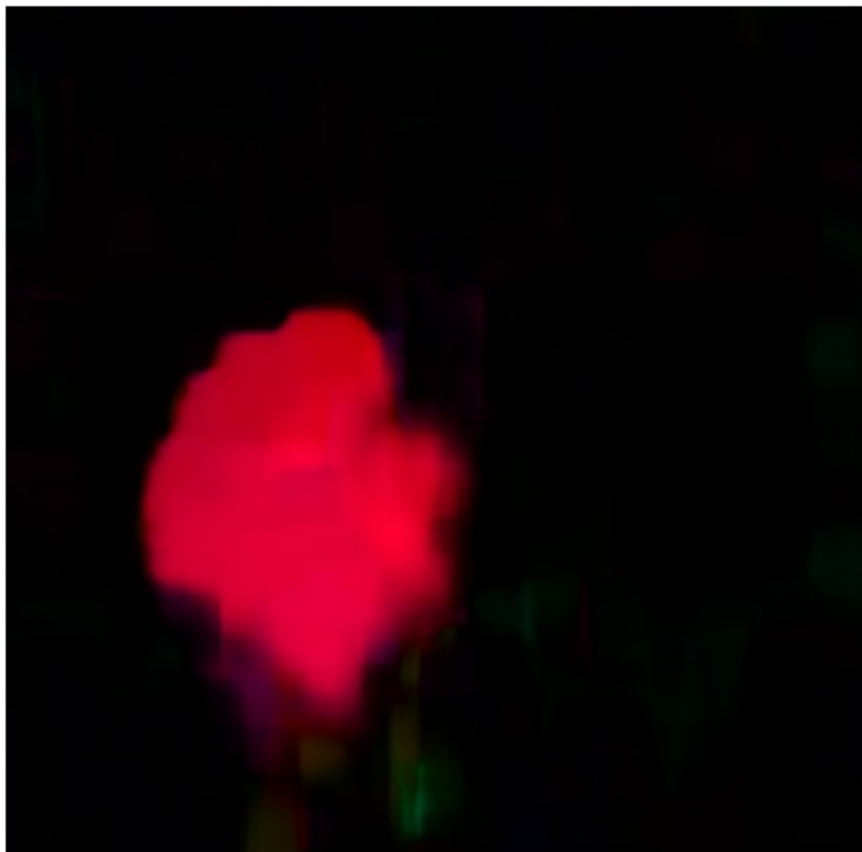
Motion Mask
