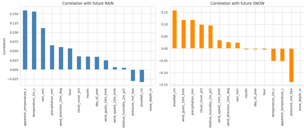
Figure 3: Correlation of features with target variable.
