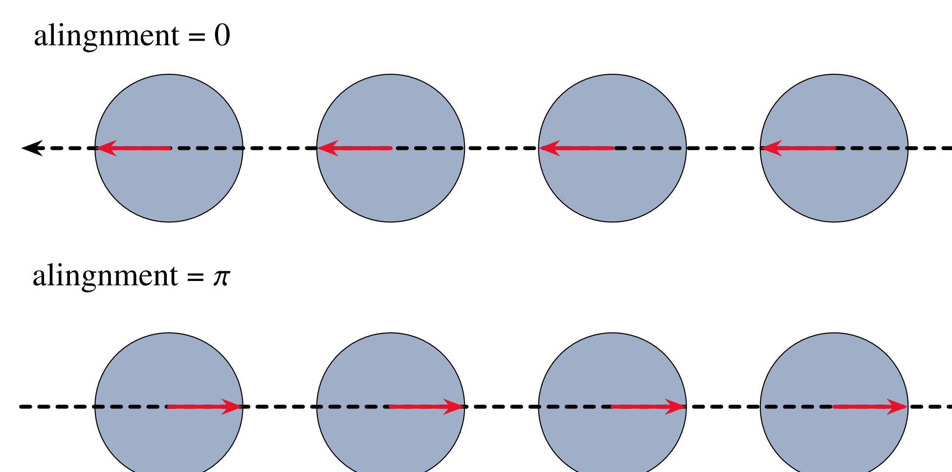
Figure 5: The schematic for superposition of the two state alignments.
