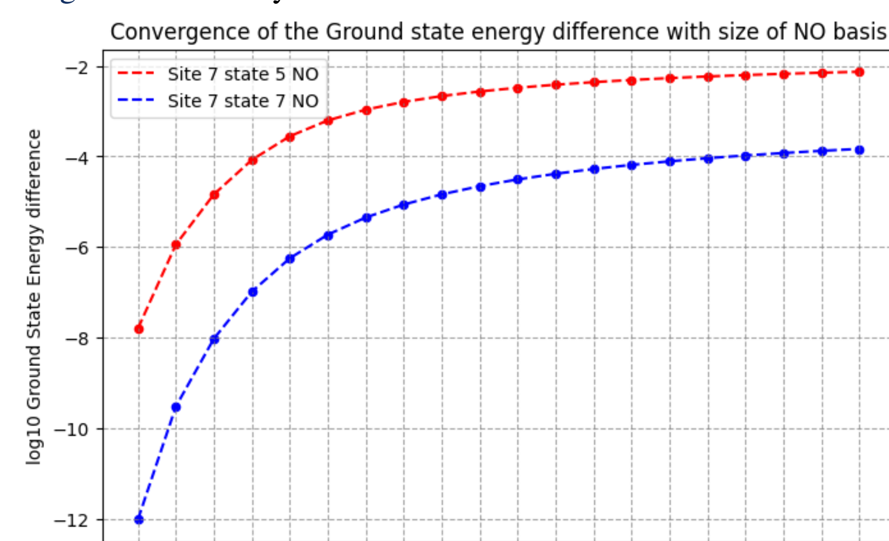
Figure 1: Accuracy of the NO with 5 and 7 NO basis truncation.
