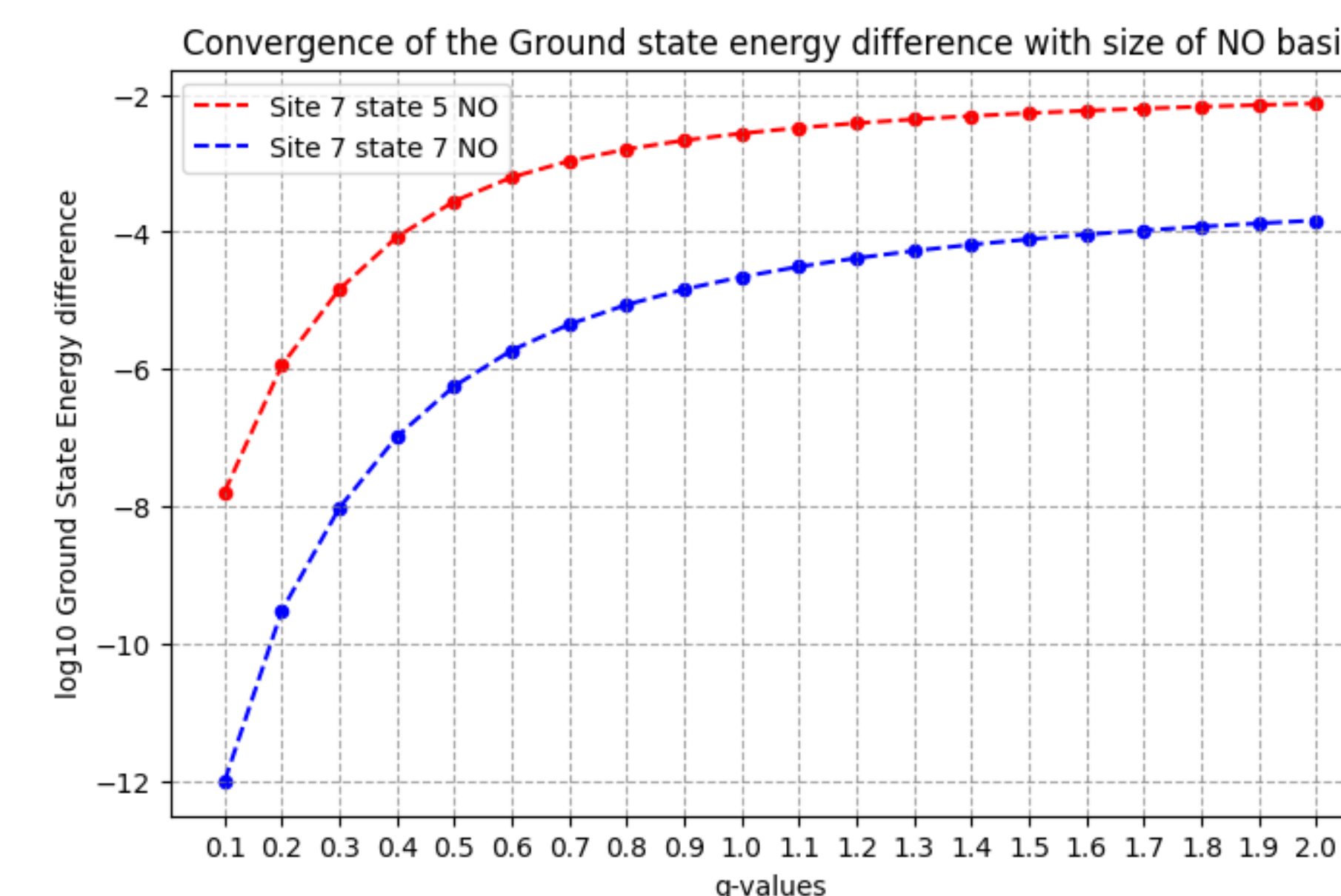
Figure 4: As g increases the CCC results love accuracy.
